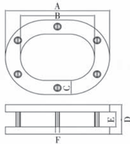
Hawse Pipe
